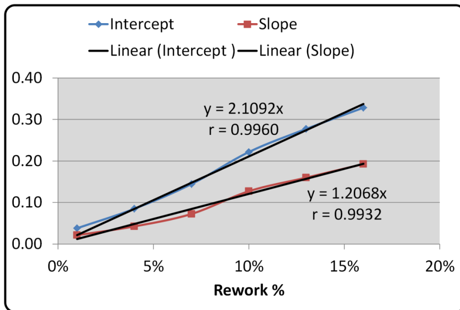
Figure 8. Linear Model
