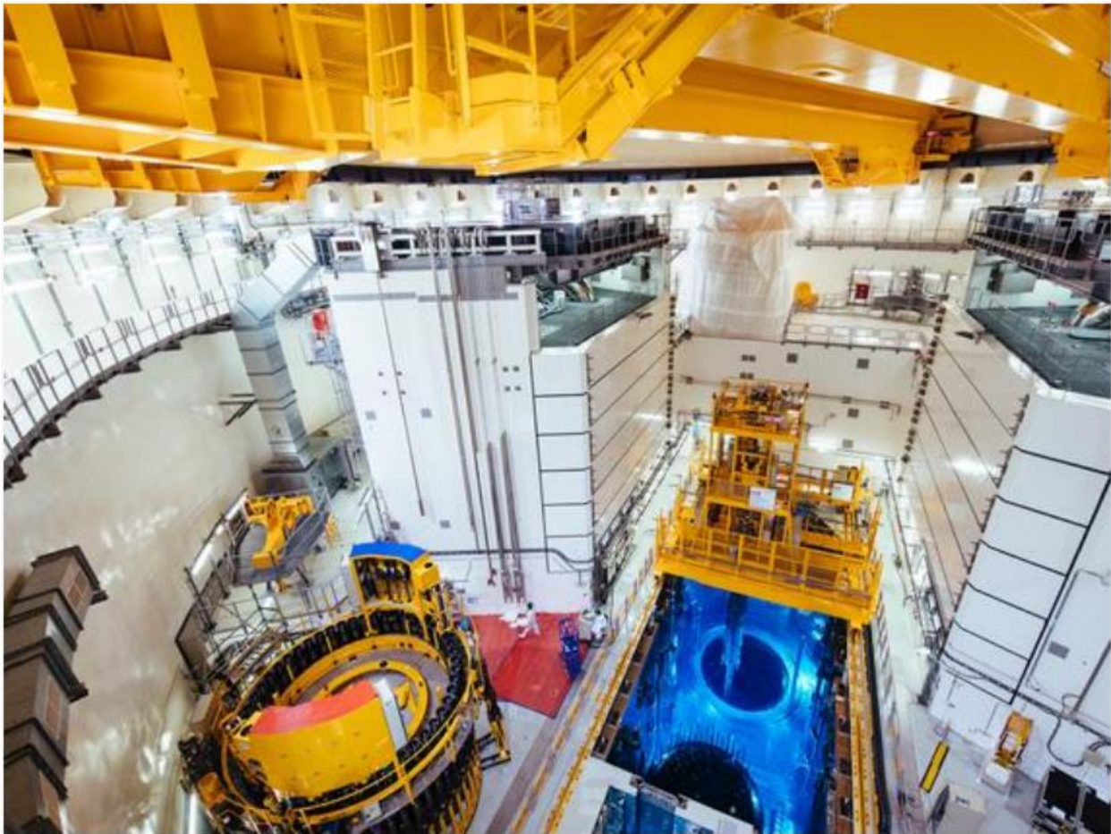
Nuclear fuel loading is about to commence in Olkiluoto 3 reactor building (photo courtesy TVO)
