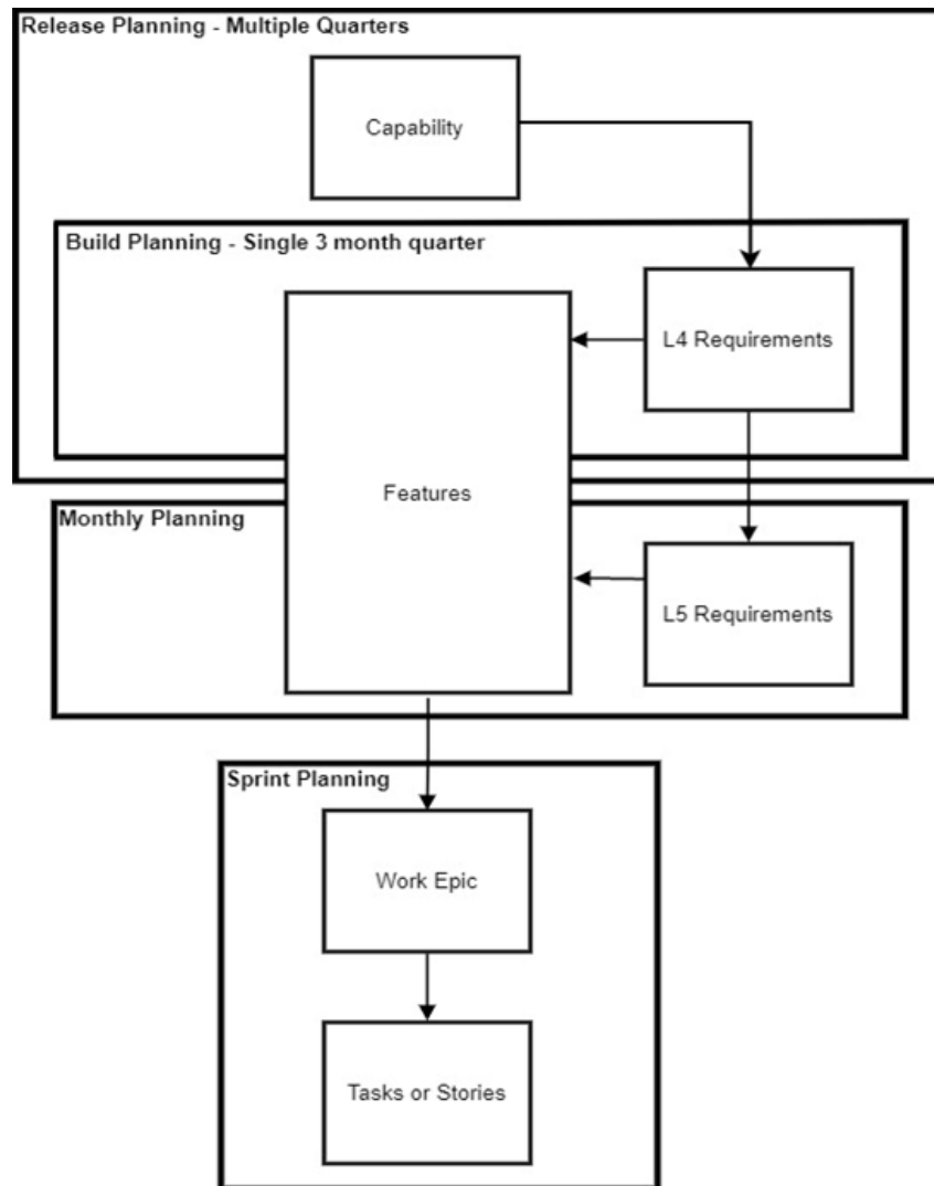
Figure 2: Release and Build Planning
